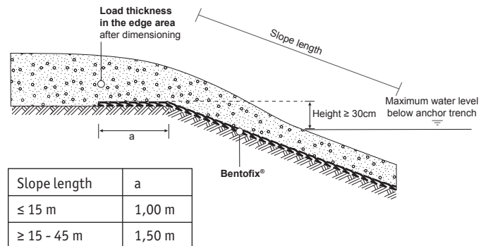
Fig. 8 a Minimum dimensions for structural integration at the crest of the slope
