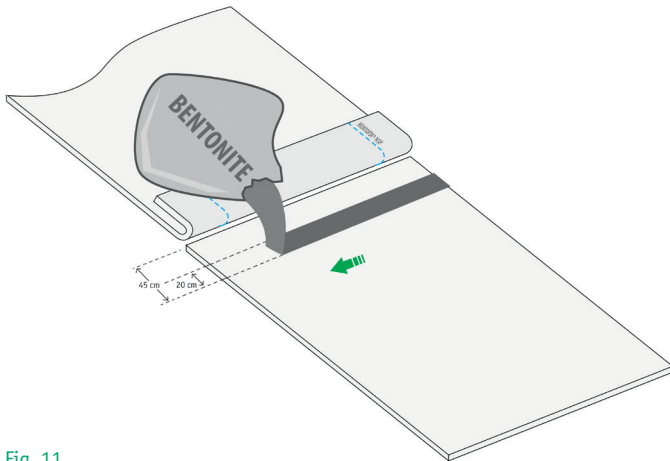
Fig. 11 Placing of bentonite onto the overlap
