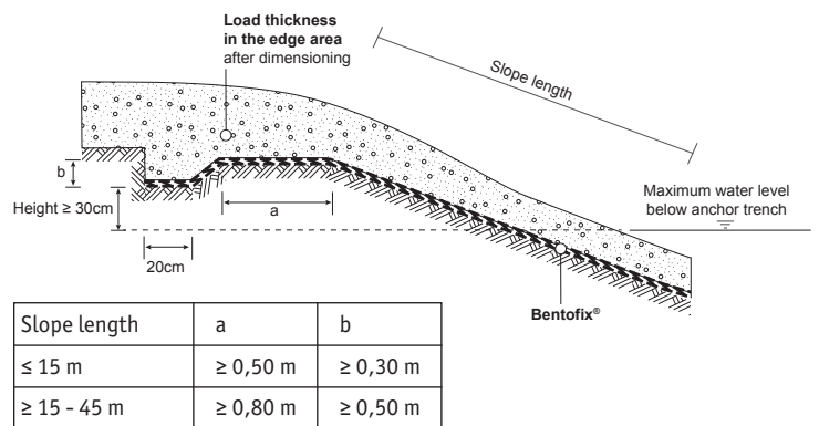
Fig. 8 b Minimum dimensions for structural integration at the crest of the slope
