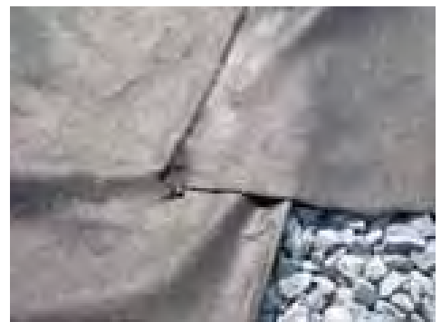
Fig 7: Overlap Geotextile by minimal 300mm or more.
