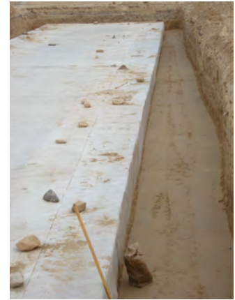
Fig. 23 Vibratory compaction of side backfill is always required , regardless of what backfill material is used.
