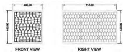
Fig 9 : Make Sure the tanks are oriented Properly and correct way in the excavation.
